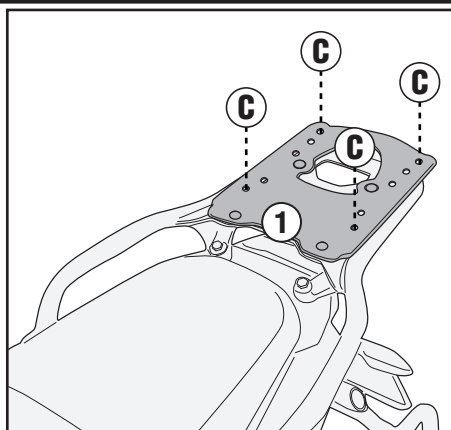
M5/M5M/M6M PLATE
